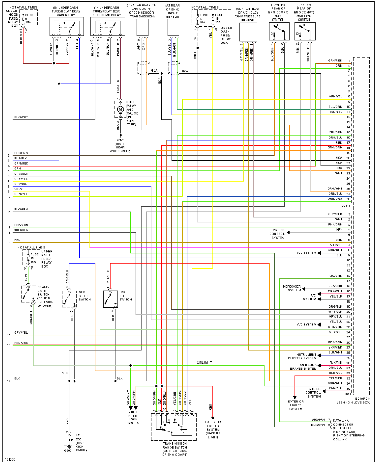
Fig. 12: 2.0L, Engine Performance Circuits (3 of 3)
