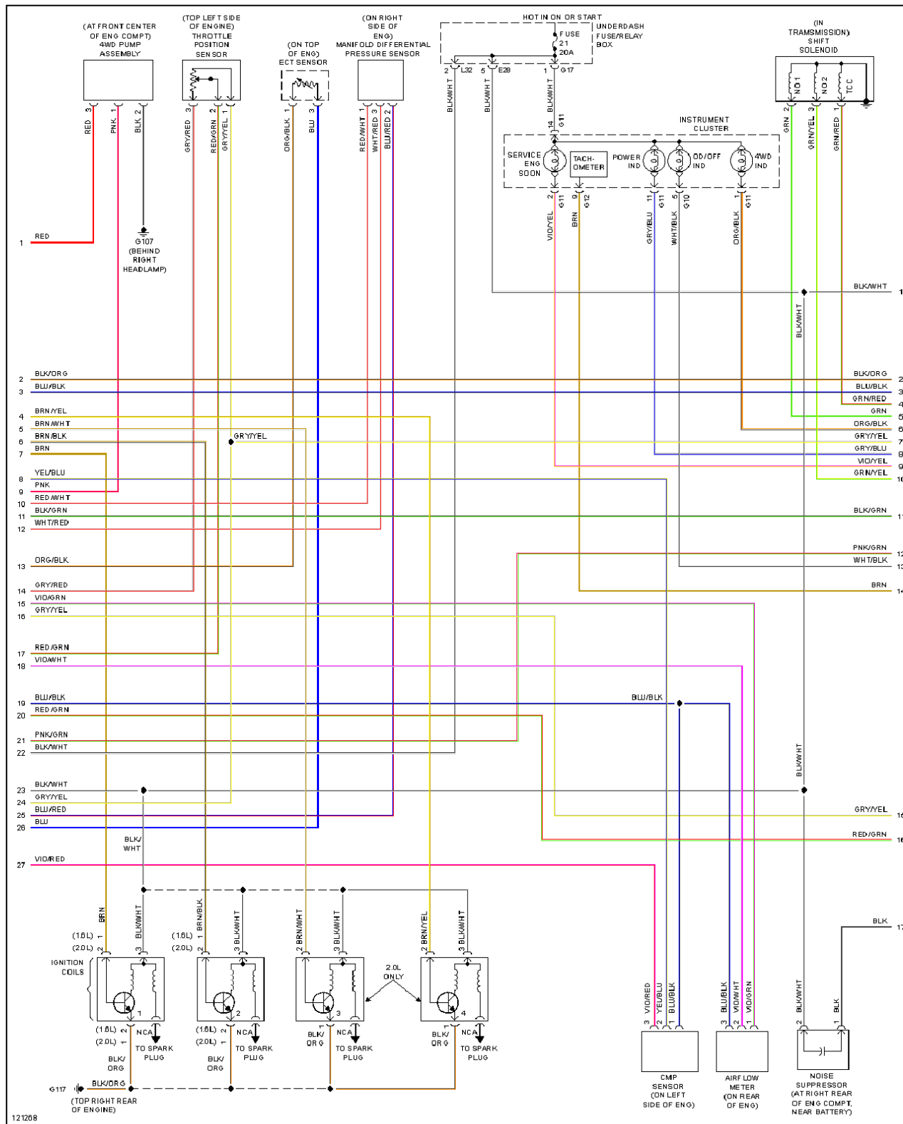
Fig. 11: 2.0L, Engine Performance Circuits (2 of 3)
